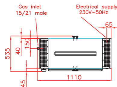
Top view Rotisserie and base on casters
