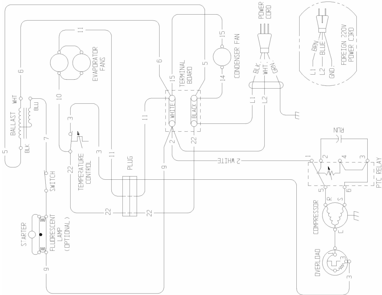
WIRING DIAGRAM MODEL : SKR48
