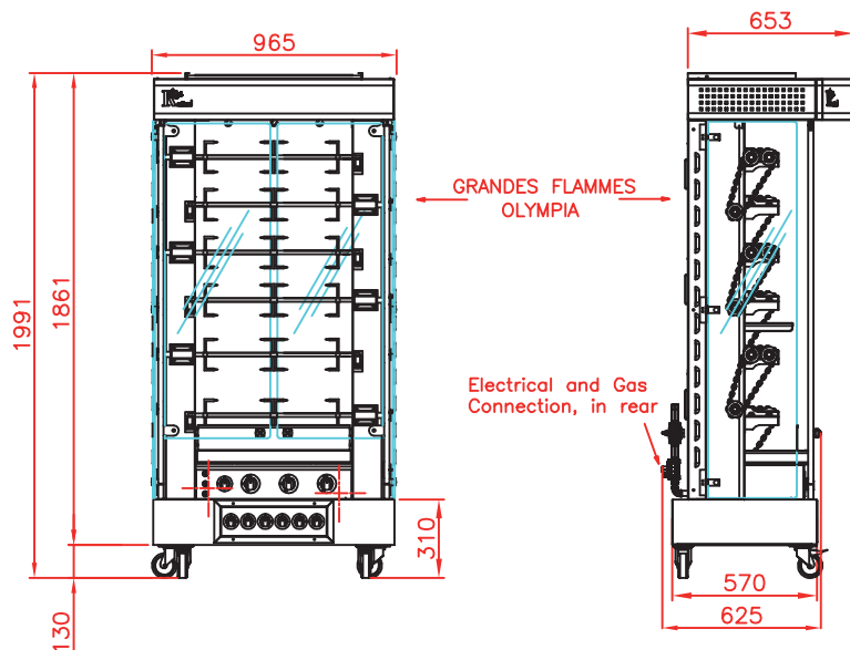
Front view Rotisserie with roof and base on casters
