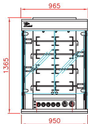
Front view Rotisserie with roof and base on casters (optional)
