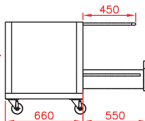
Heated base cabinet with drawers (Optional)
