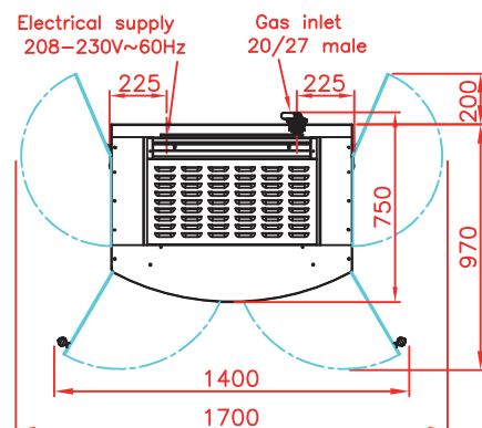
Top view Rotisserie with roof and base on casters (optional)
